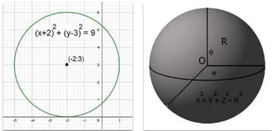
Figure 3.22 – Mathematical formulas of some geometrical lines and forms
