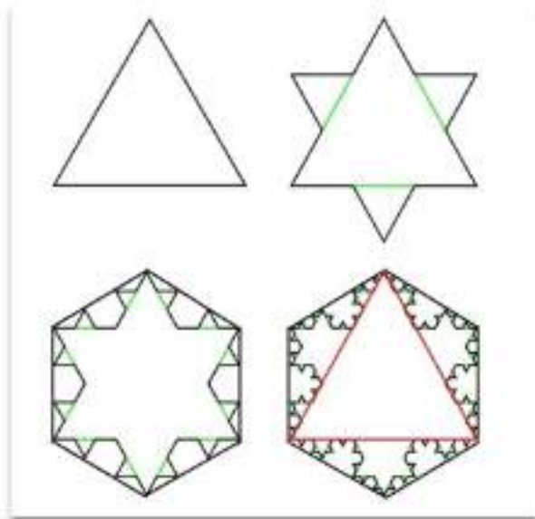
Figure 3.24 – Koch Snowflake
