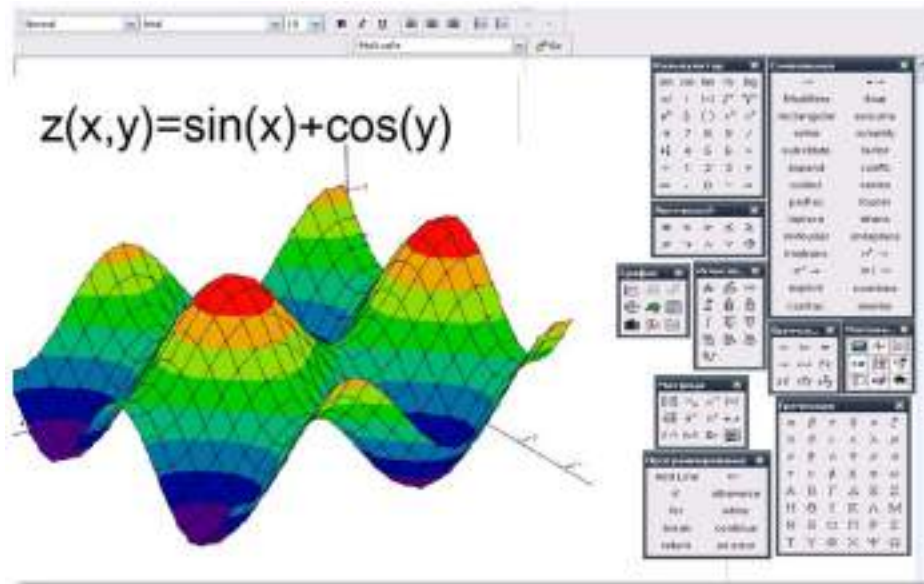
Figure 3.7 – MathCad Visualisation
